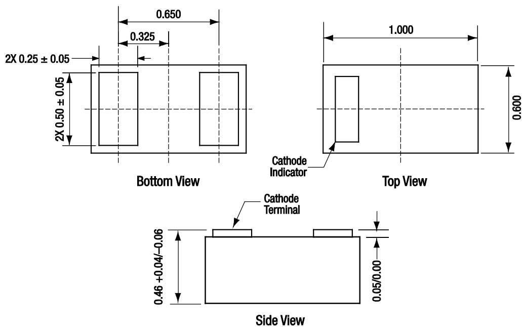
Figure 5. SMP1345-040LF Package Dimensions
