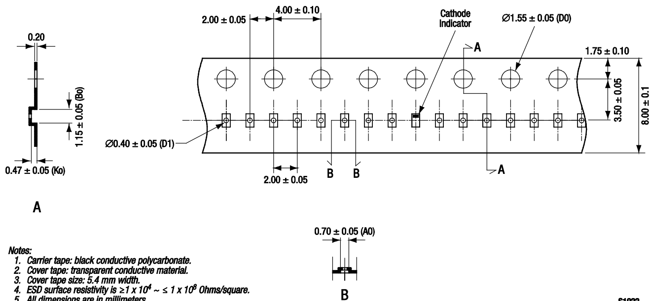
Figure 6. SMP1345-040LF Tape and Reel Dimensions
