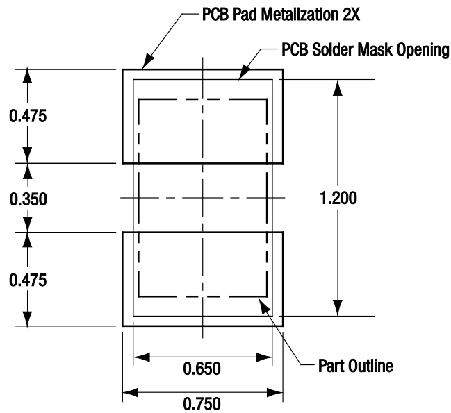
Figure 3. SMP1345-040LF PCB Layout Footprint
